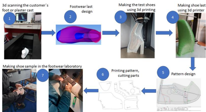
Fig.1 The main stages of process of creating the orthopedic shoes and footwear for the personal parameters
