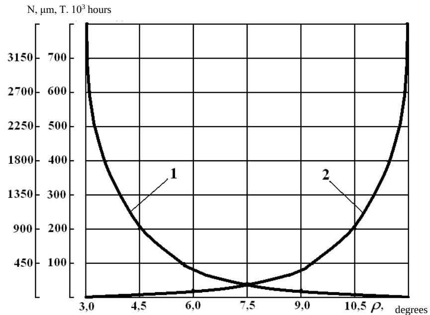
Figure. The effect of friction on the life cycle of the KO-2 circular knitting machine stitch cams (curve 1) and their working surface wear (curve 2) at T = 10 \cdot 10^3 hours
